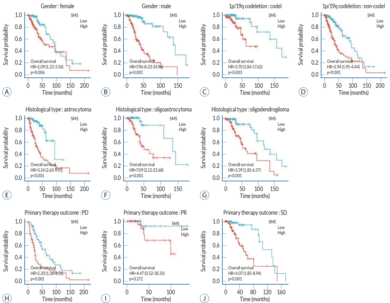
Supplementary Fig. 5. Kaplan-Meier analysis of overall survival for the remaining ten representative subgroups based on gender (A and B), 1p/19q co-deletion (C and D), histological type (E-G), and initial treatment outcome (H-J). SMS : spermine synthase, HR : hazard ratio, PD : progressive disease, PR : partial response.
