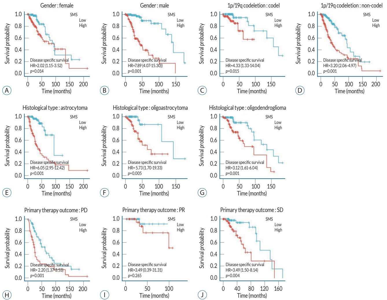
Supplementary Fig. 7. Kaplan-Meier analysis of disease-specific survival (DSS) for the remaining ten representative subgroups based on gender (A and B), 1p/19q co-deletion (C and D), histological type (E-G), and initial treatment outcome (H-J). SMS : spermine synthase, HR : hazard ratio, PD : progressive disease, PR : partial response, SD : stable disease.
